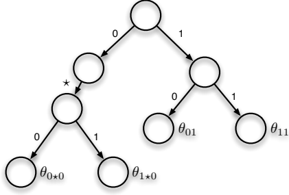
Figure 5. A 1-skip prediction suffix tree.
